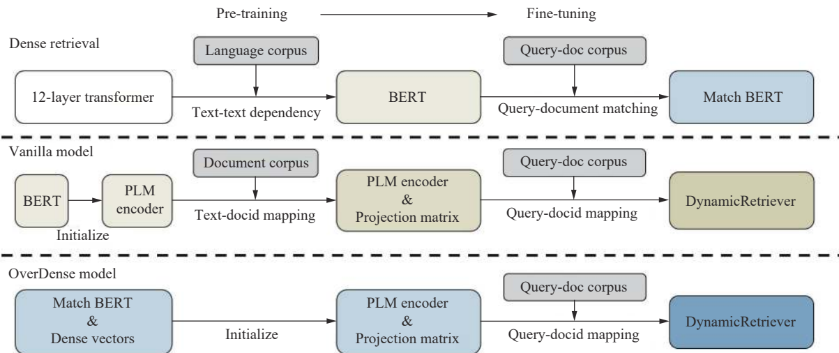
Fig. 2 Model training workflows of dense retrieval and two variant models of DynamicRetriever
