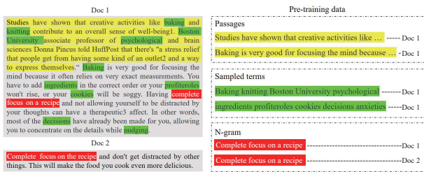
Fig. 3 Pre-training tasks of the Vanilla model
